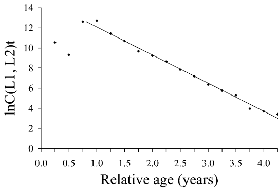
Fig. 5. Catch curve for the estimation of Z (total instantaneous mortality).
