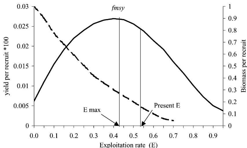
Fig. 8. Yield per recruit and biomass per recruit curves for B. auritus according to the exploitation rate and length at recruitment.
