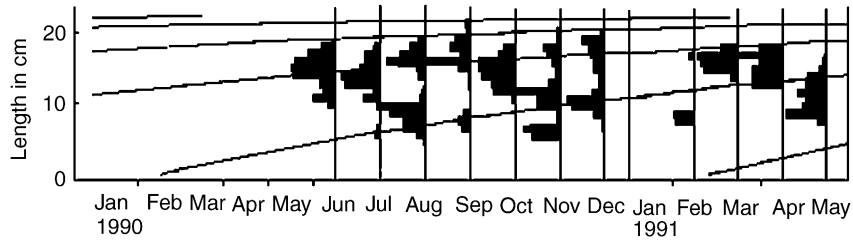
Fig. 4. Growth curves of B. auritus estimated by ELEFAN superimposed on length–frequency histograms.
