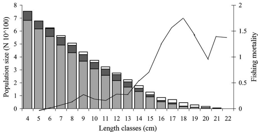
Fig. 6. VPA graph showing catches, survivors and fishing mortality for the various length classes.
