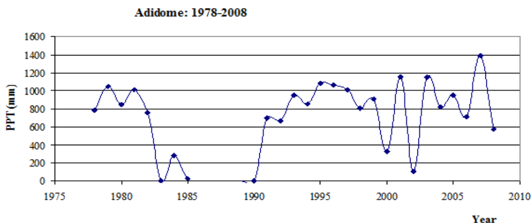
Fig. 3. Variation in 30-year annual rainfall total in North Tongu District
